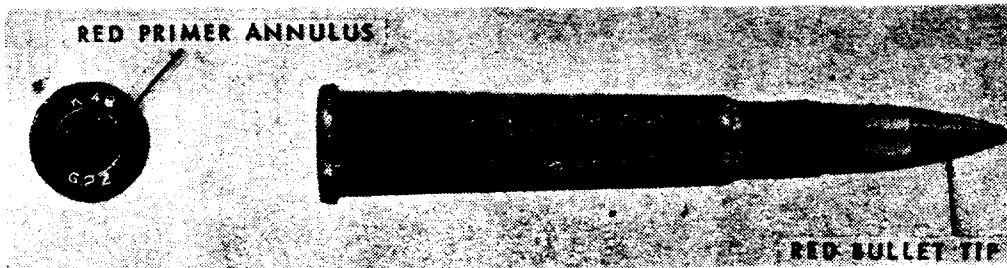
Figure 15. Tracer Cartridge With Bullet Tip and Primer Annulus Color Identification
