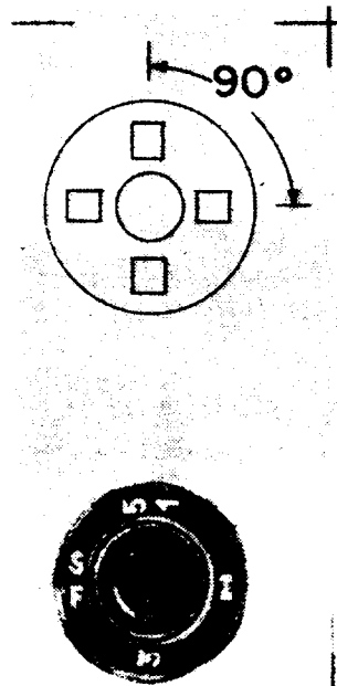
Figure 12. Four-Element Headstamp
