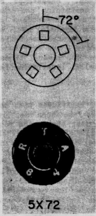
Neg. 525243 Figure 13. Five-Element Headstamp
