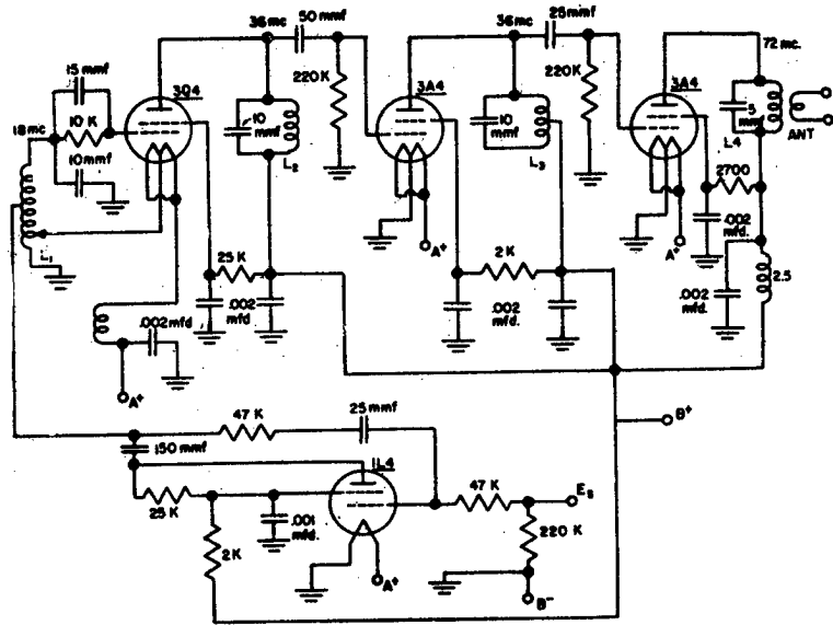
Fig. 4 FM-1 Transmitter
