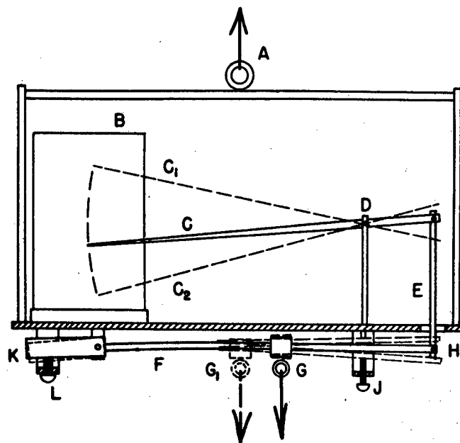
Figure 38. Ballast-recording meter.
