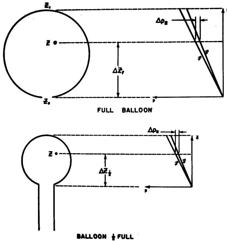
Figure 24. Comparison of pressure head across partially and fully inflated balloons.
