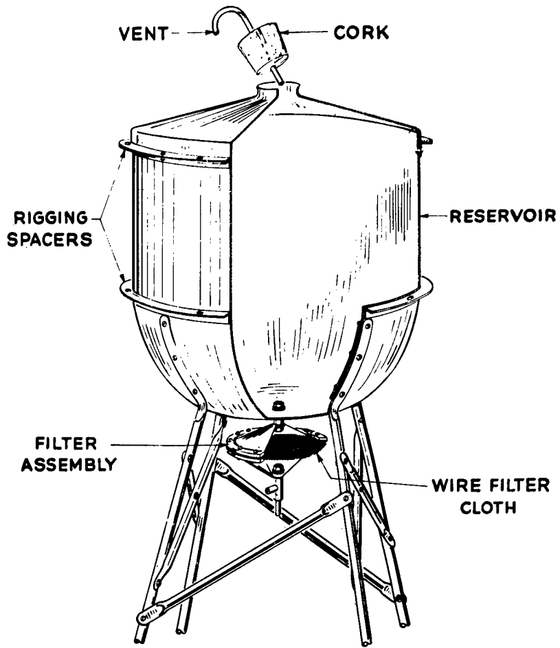
BALLAST RESERVOIR
