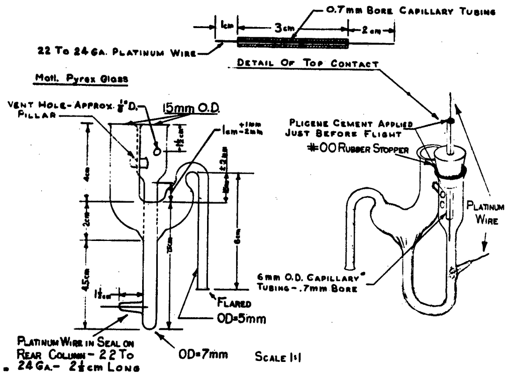
Figure 37. Automatic siphon.
