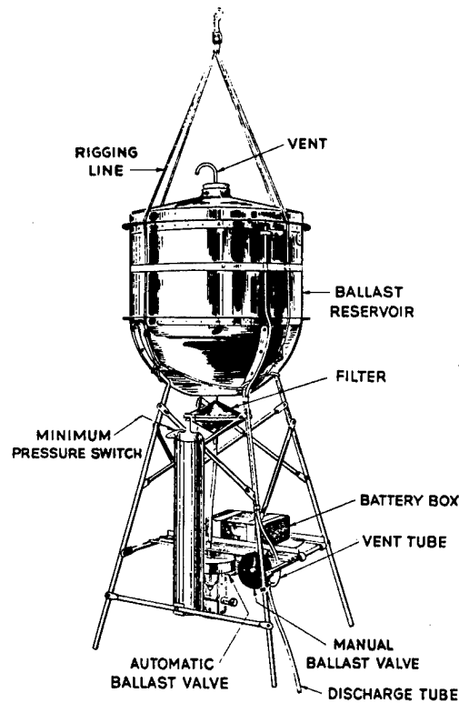
FIG. 3. Ballast-release assembly.
