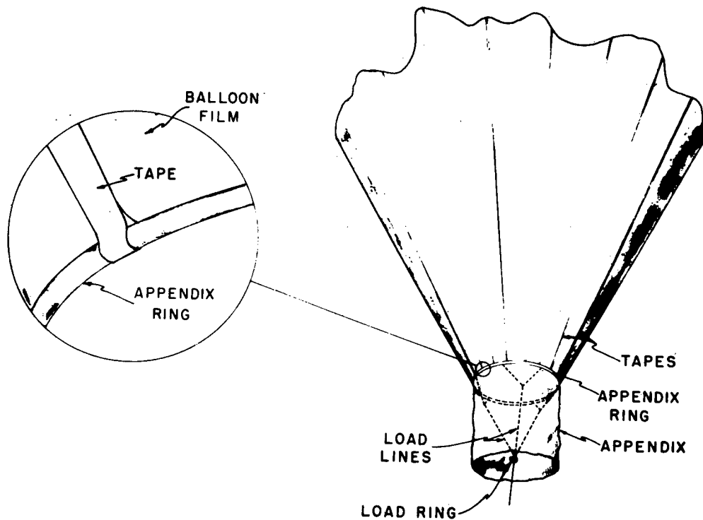
Figure 6. Appendix detail, polyethylene balloon.
