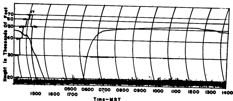
NYU BALLOON PROJECT FLIGHT 82 Barograph Record Of G.M.20' Plastic Balloon With 534 gm/hr Fixed Ballast Leak
