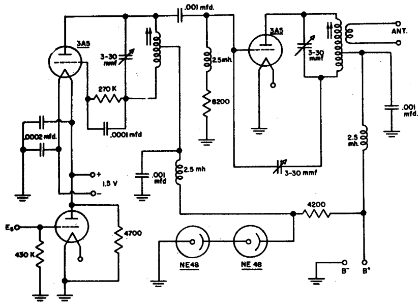
Fig. 5 FM-2 Transmitter
