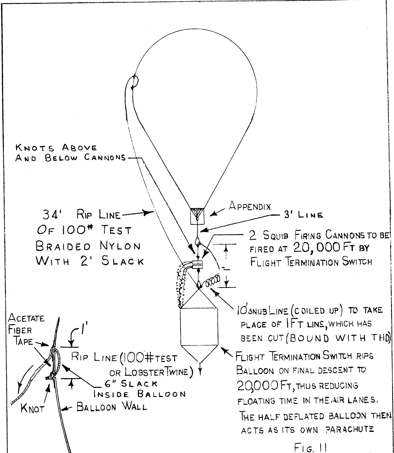
DETAIL OF RIP LINE INSERT INTO BALLOON
