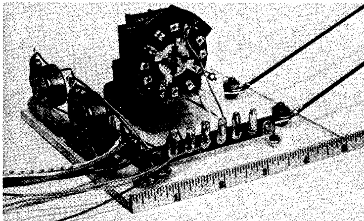
Figure 36. Temperature programming switch.
