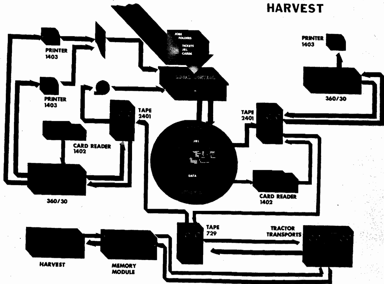
The IBM HARVEST System
