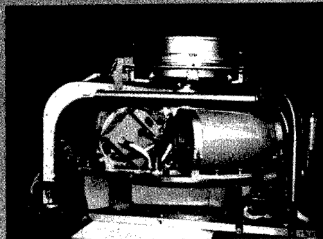
KOSMOS-936 CENTRIFUGE. TWO SUCH UNITS WERE OPERATED CONTINUOUSLY DURING THE 18.5 DAY FLIGHT, PROVIDING ARTIFICIAL GRAVITY (1-G) AND LIFE SUPPORT FOR FIVE RATS EACH.
