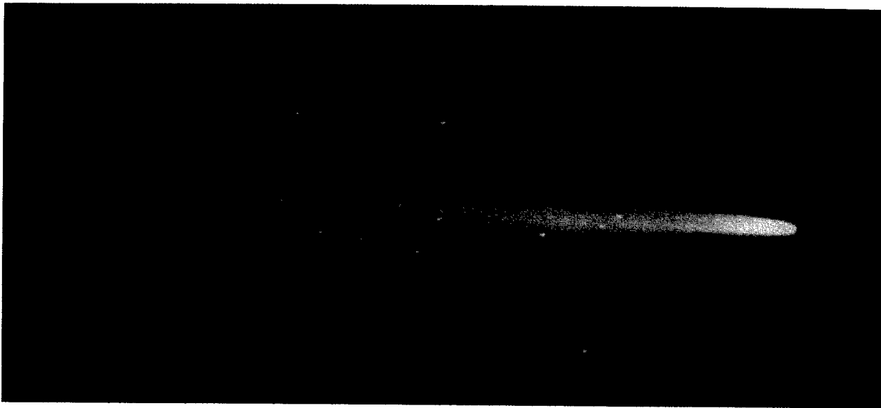
View of Comet Halley, taken in May 1910
