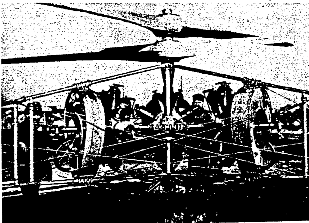
Close-up of engines and counterrotating propellers of von Kármán helicopter.
