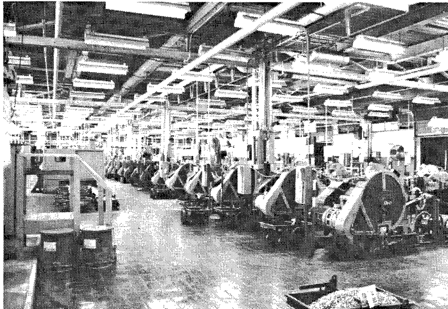
Figure 105. Building 11: Interior of Lead Extrusion and Swaging Building.
