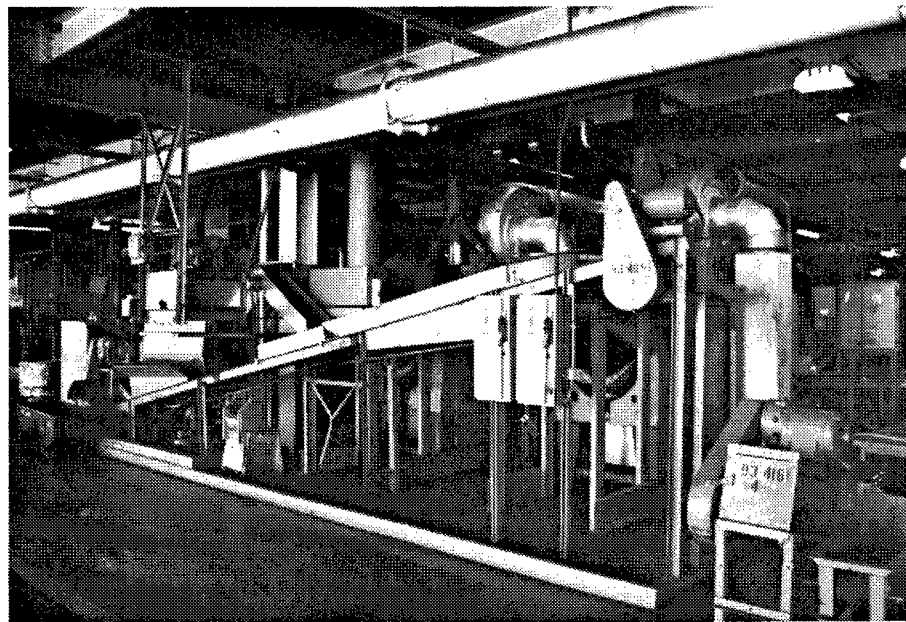
Figure 47. Building 3: Wash, Rinse, and Dry Machine manufactured by Colt's Manufacturing.
