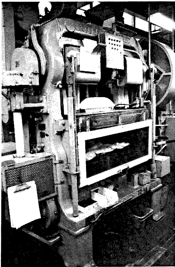
Figure 17. Building 2: Bullet Assembly Machine manufactured by Waterbury-Farrel.
