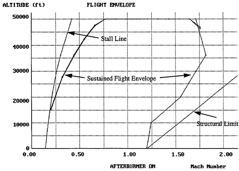
Figure C.1—Flight Envelope
