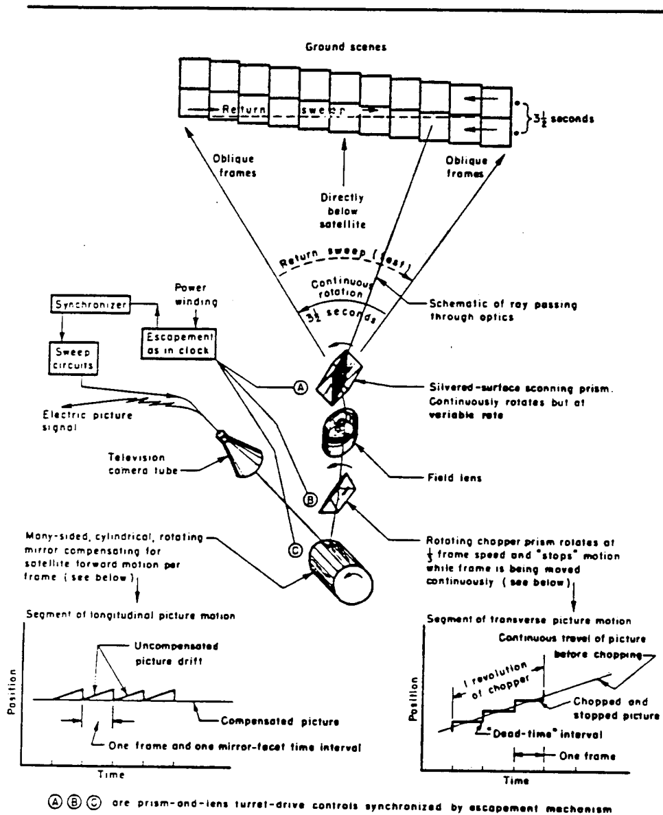
Fig. 14—Schematic illustration of optical-scanning system
