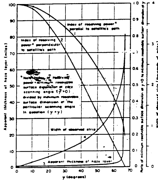
Fig. 46—Scanning angle, \gamma , vs apparent thickness of haze layer, index of resolving power perpendicular and parallel to the satellite's path, and width of observed strip
