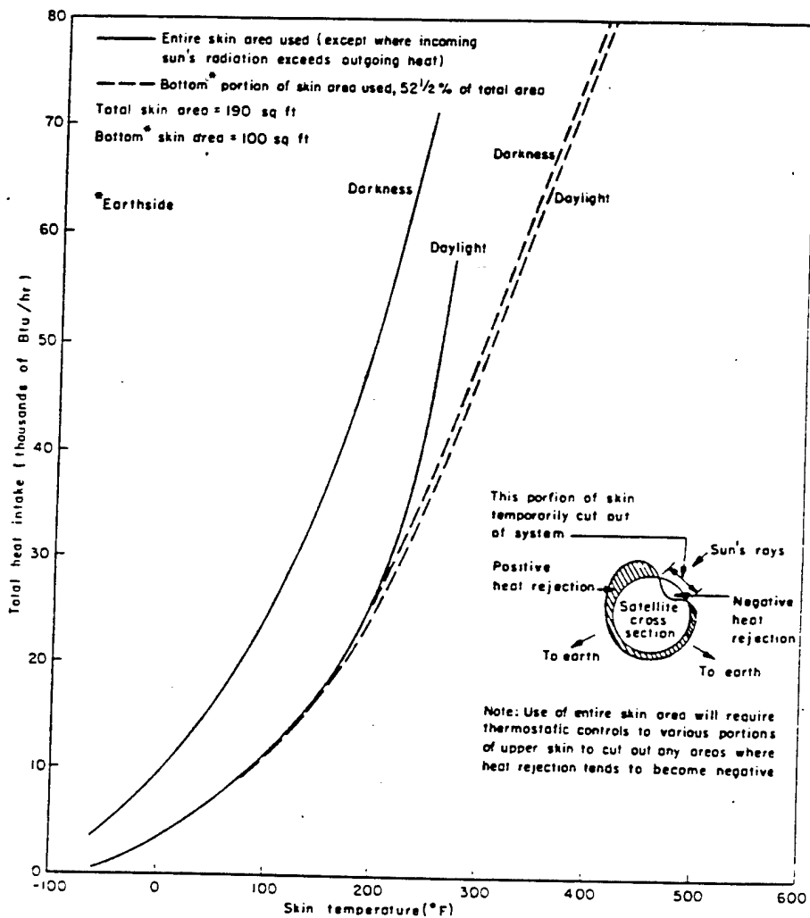
Fig. 53—Total heat that can be dissipated by radiation from skin of 1000-lb-payload satellite vs temperature of skin for two cases
