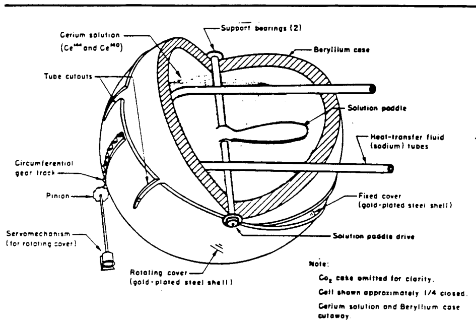
Fig. 29—Cerium cell with controlled-heat input to the heat-transfer fluid
