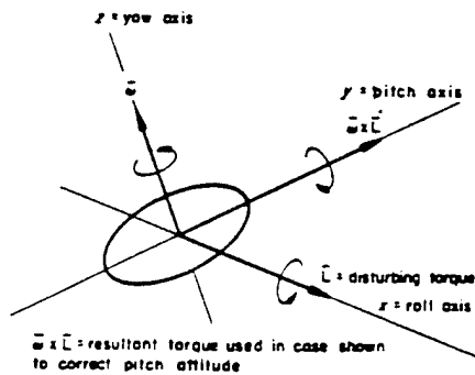
Fig. 26—Gyro precession
