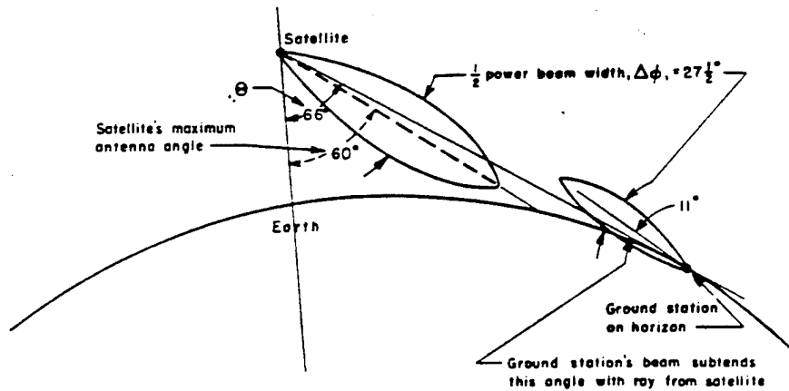
Fig. 23—Schematic diagram of satellite-tracking transmission angles
